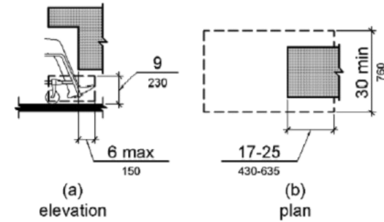
Figure 306.2 Toe Clearance
