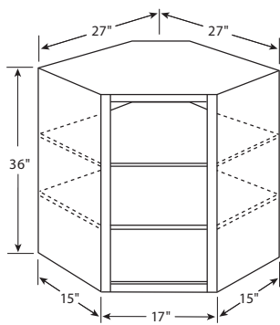
Corner Wall Cabinet 36" High x 15" Deep, 1 Door
